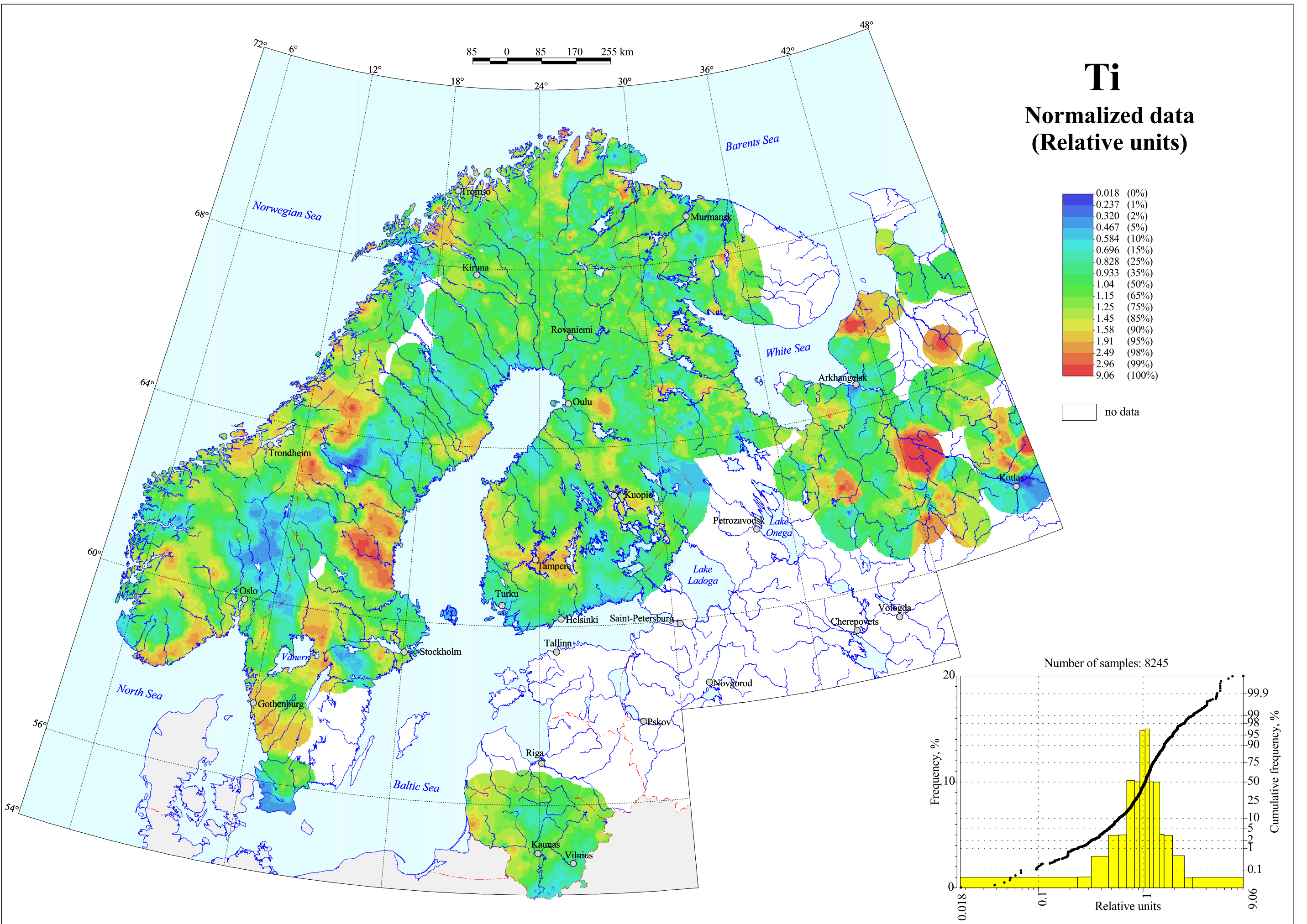
Titanium in Till, Grain Size <0.06 mm
